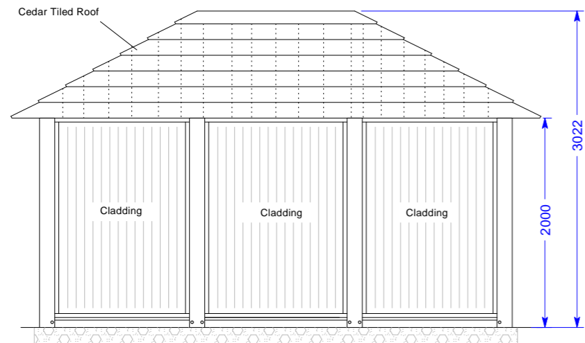
Back Elevation View C
