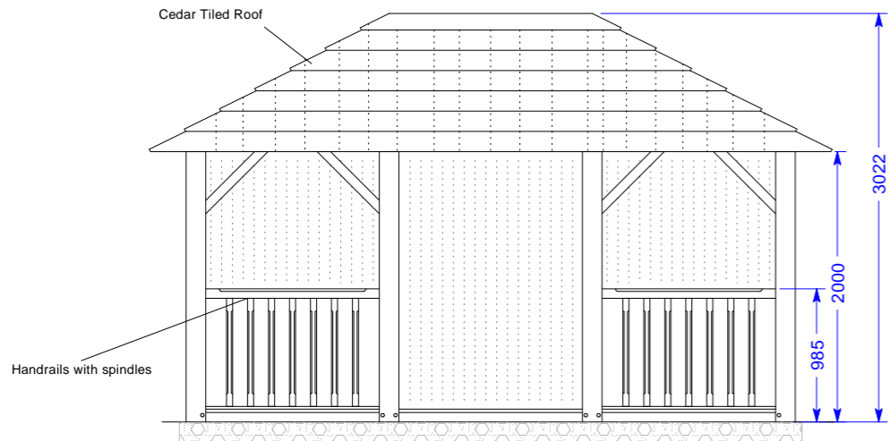
Front Elevation View A
