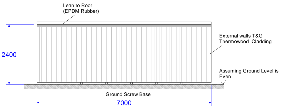
Elevation View C
