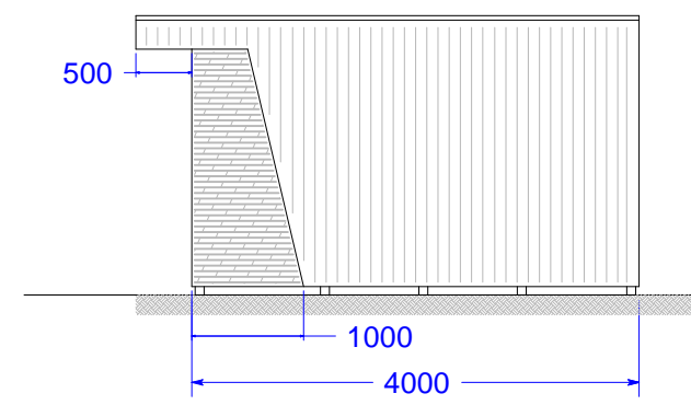
Elevation View D
