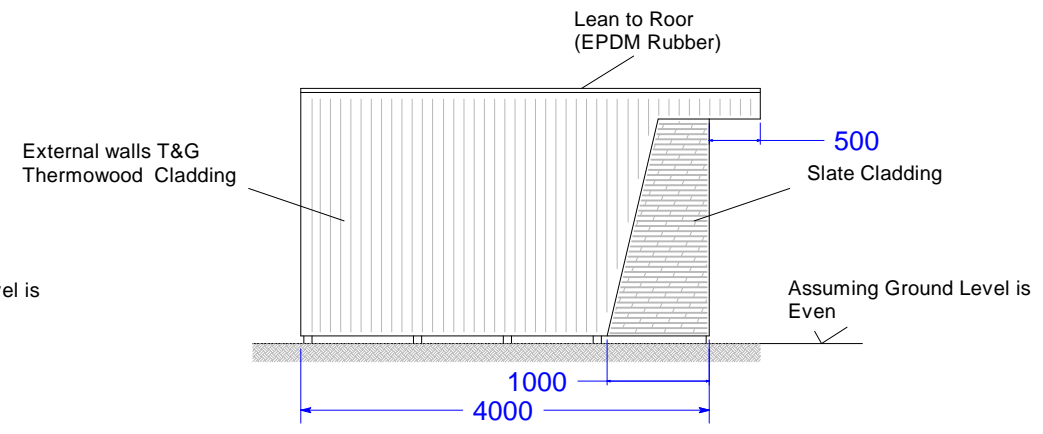
Elevation View B
