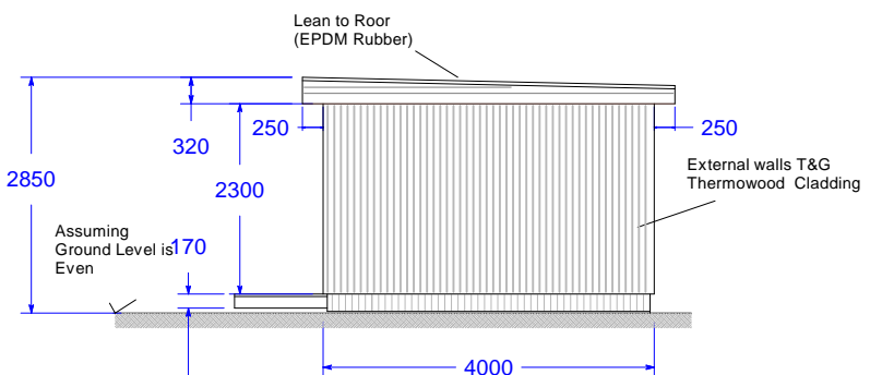
Elevation View D
