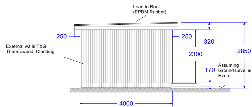
Elevation View B
