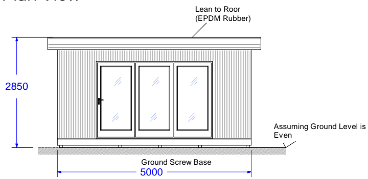
Elevation View A
