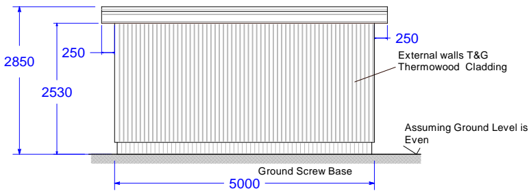
Elevation View C
