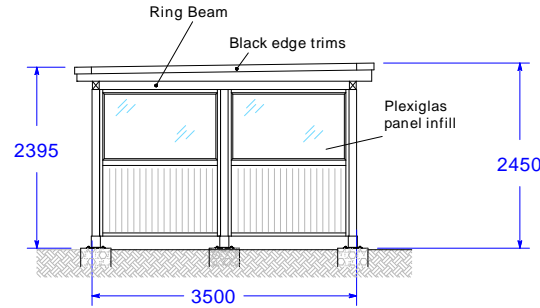
Left Elevation View
