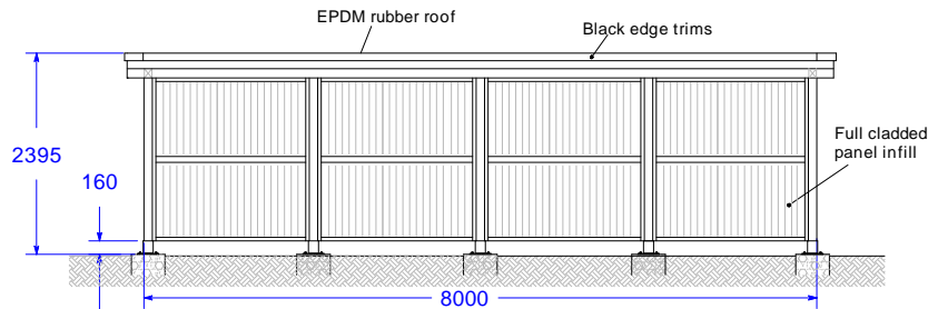
Back Elevation View
