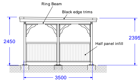
Right Elevation View
