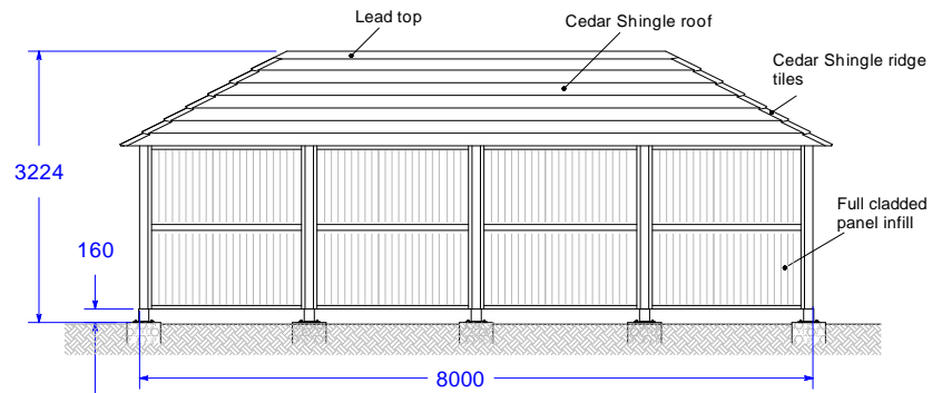
Back Elevation View
