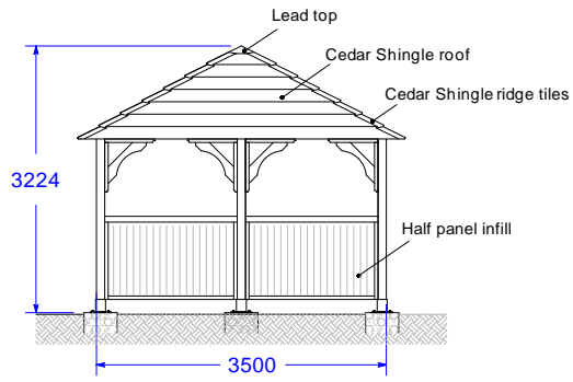
Right Elevation View
