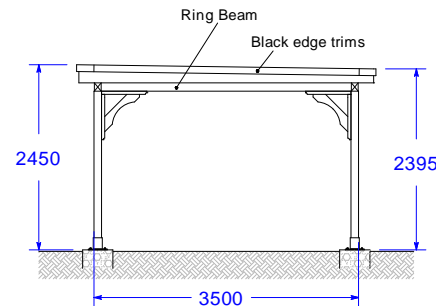
Right Elevation View
