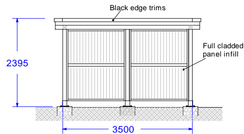
Back Elevation View
