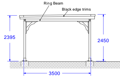
Left Elevation View
