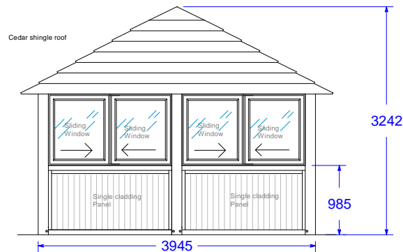
Elevation View Right
