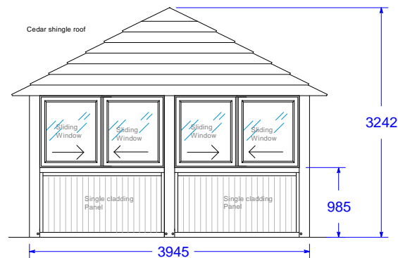
Elevation View Left
