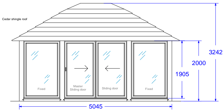
Elevation View Front
