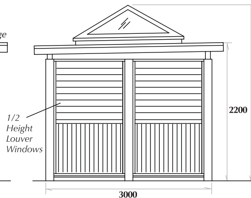
LEFT ELEVATION
