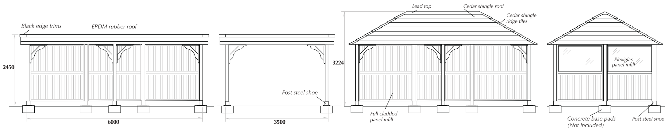
FRONT ELEVATION
